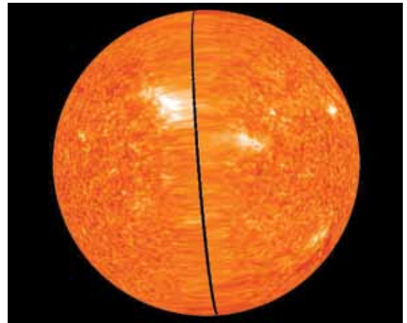
This image, taken February 2, 2011, of the far side of the Sun based on STEREO data, still shows a small gap between the STEREO Ahead and Behind data. On February 6, the spacecraft achieved 180-degree separation, closing the gap. (Credit: NASA)
