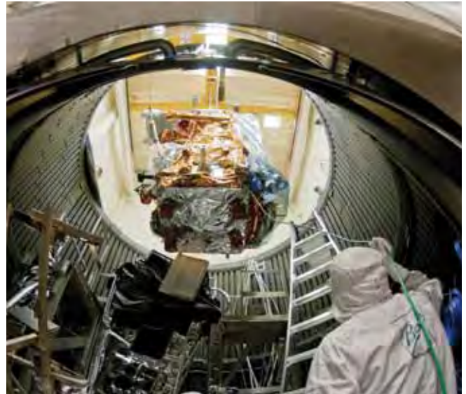
An engineer from Ball Aerospace guides the NPOESS Preparatory Project (NPP) satellite into a thermal vacuum chamber for environmental testing. Once the satellite is inside, the air is pumped out of the chamber and temperature extremes are applied to replicate orbit conditions. Completing a project like NPP requires dedication, teamwork, and attention to detail from all participants—NASA, contractors, and partners. (Credit: Ball Aerospace)
