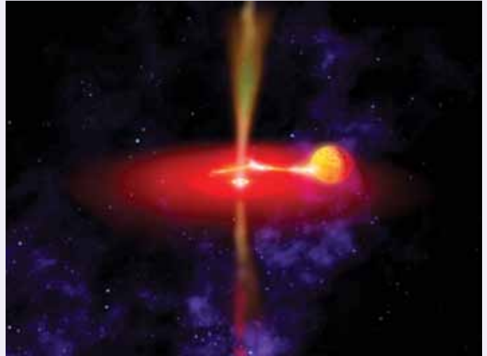
Astronomers using NASA's Wide-field Infrared Survey Explorer (WISE) have captured rare data of a flaring black hole, revealing new details about these powerful objects and their blazing jets. This artist's concept illustrates what the flaring black hole called GX 339-4 might look like. Infrared observations from WISE reveal the best information yet on the chaotic and extreme environments of this black hole's jets. GX 339-4 likely formed from a star that exploded. It is surrounded by an accretion disk (red) of material being pulled onto the black hole from a neighboring star (yellow orb). Some of this material is shot away in the form of jets (yellow flows above and below the disk). The region close in to the black hole glows brightly in infrared light. Read more about this story. (Credit: NASA)
